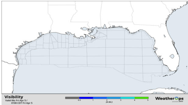
Visibility Forecast 1200 CT Apr-05
