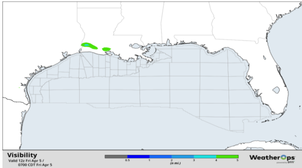
Visibility Forecast 1800 CT Apr-05
