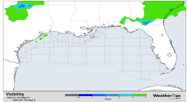
Visibility Forecast 1500 CT May-09
