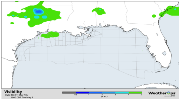
Visibility Forecast 1800 CT May-09
