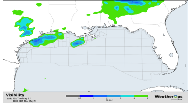
Visibility Forecast 0900 CT May-09
