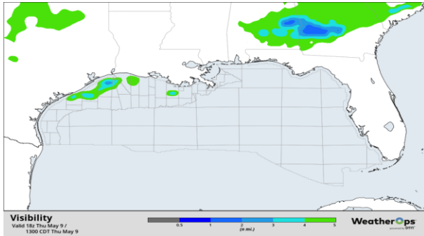
Visibility Forecast 1200 CT May-09
