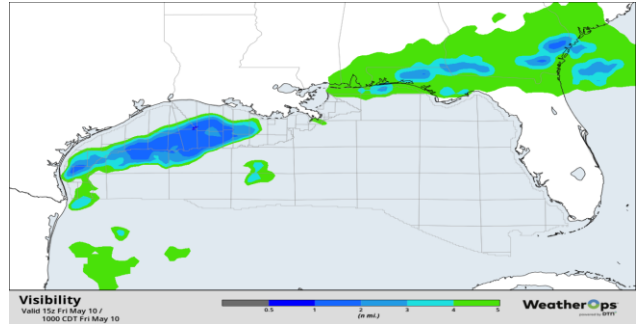
Visibility Forecast 0900 CT May-10
