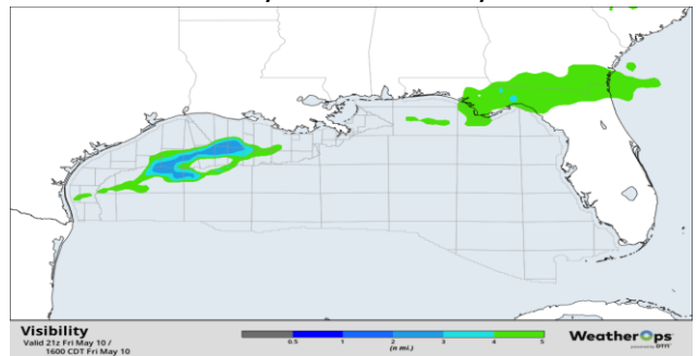
Visibility Forecast 1500 CT May-10
